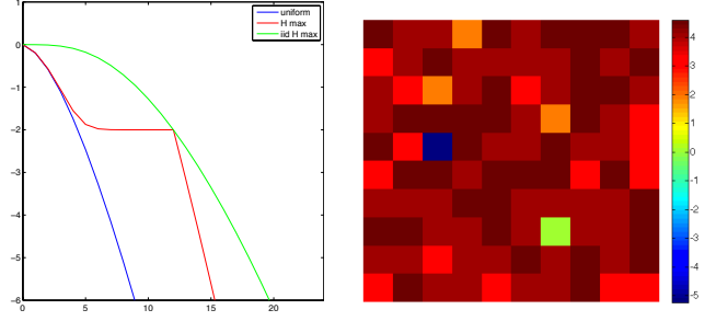
Fig. 2 On the left, graphs of k \mapsto \log_{10} \mathbb{P}_P(k(R; S) \geq k) for P being respectively the uniform distribution U (blue curve), the distribution in \mathcal{P}_R that has maximum entropy (red curve) and the distribution in \mathcal{P}_R \cap \mathcal{I} that has maximum entropy (green curve). On the right, image of the \log(\text{NFA}_P(R_i)) for all regions R_i when P is the distribution in \mathcal{P}_R \cap \mathcal{I} with maximum entropy. See the text for more details.
