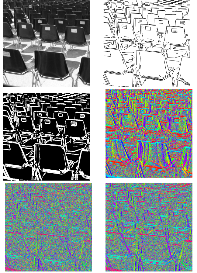
Fig. 7 From left to right, top to bottom: the original Chairs image I^0 of size 512 \times 512 pixels, the output of the LSD, the whole output rectangles of the LSD, the orientation field \theta^0 , a sample from P_0 and a sample from Q_0 .
