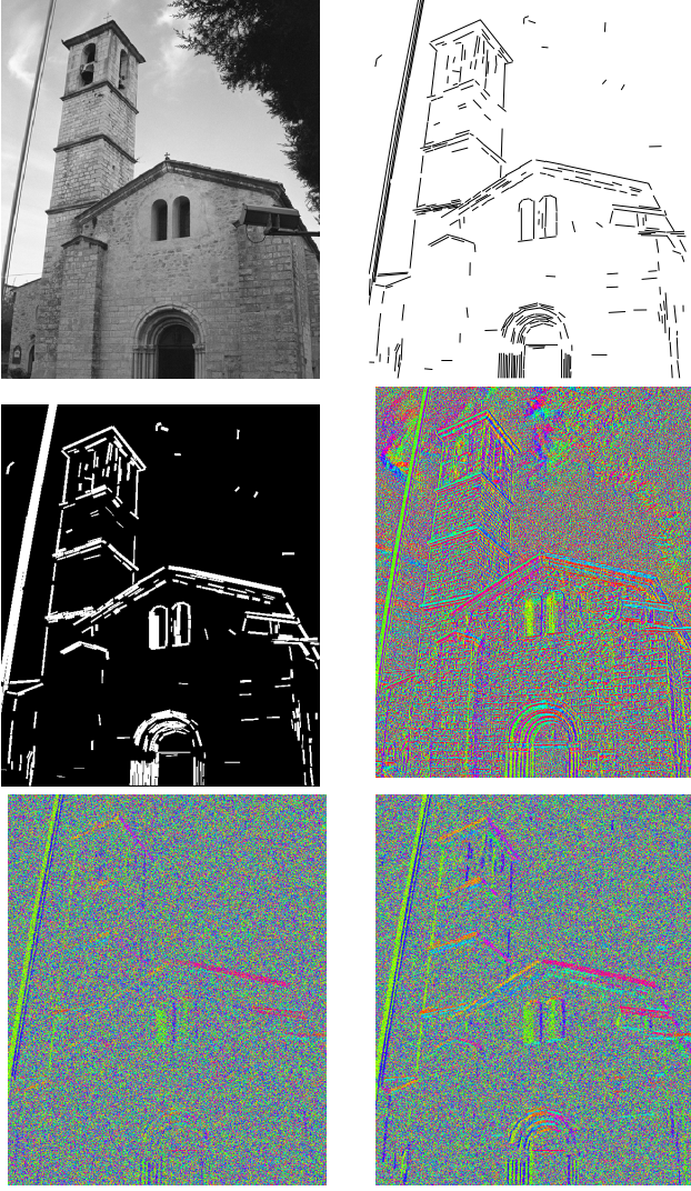
Fig. 8 From left to right, top to bottom: the original Valbonne image I^0 of size 539 \times 648 pixels, the output of the LSD, the whole output rectangles of the LSD, the orientation field \theta^0 , a sample from P_0 and a sample from Q_0 .
