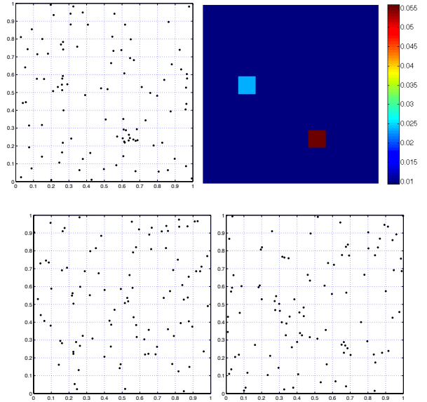
Fig. 3 Top left: the initial set of points s^0 = \{x_j^0\}_{1 \leq j \leq n} and the regions R_i (delimited by the dashed squares). Top right: value of p_{P_0}(R_i) for each region R_i where P_0 is the maximum entropy distribution such that the points are independent and such that no regions are (\varepsilon, P_0) -meaningful for s^0 , it is defined by (4). Bottom: two samples of n = 100 points with the law P_0 . These samples look a bit more “structured” than uniform samples but they don’t have the same “look and feel” as the initial set of points s^0 = \{x_j^0\}_{1 \leq j \leq n} . See the text for more detailed comments.
