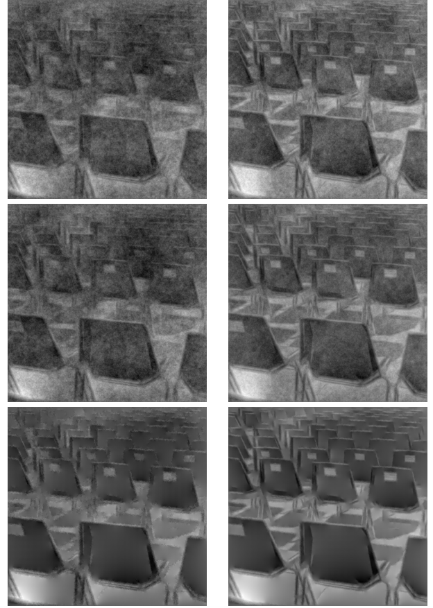
Fig. 10 The original image I^0 was here the Chairs image of Figure 7. On the left column, we show the images reconstructed from a sample of P_0 (the one shown on Figure 7) and with respectively from top to bottom R_{rand} , R_{cst} and R_{100} . On the right column, same experiment but with the sample from Q_0 .
