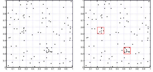
Fig. 1 Example of points and regions. Here we have a set s^0 of n = 100 points in the domain D = [0, 1]^2 , and the tested regions are small squares of side length 0.1 and delimited by the dashed lines. On the left image, one can clearly perceive that two regions are not like the others, in the sense that they contain an “unexpectedly high” number of points. On the right, we have delimited these two (\varepsilon, U) -meaningful regions (with here \varepsilon = 1 ) in red, with a line width proportional to -\log_{10}(\text{NFA}_U(R; s^0)) . The most meaningful region is the bottom right one.
