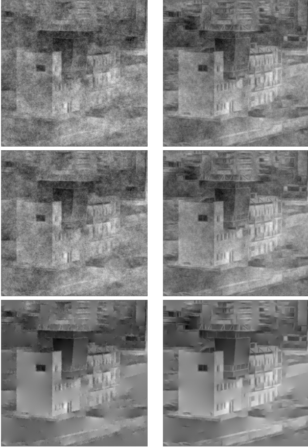
Fig. 9 The original image I^0 was here the Pirée image of Figure 6. On the left column, we show the images reconstructed from a sample of P_0 (the one shown on Figure 6) and with respectively from top to bottom R_{rand} , R_{cst} and R_{100} . On the right column, same experiment but with the sample from Q_0 .
