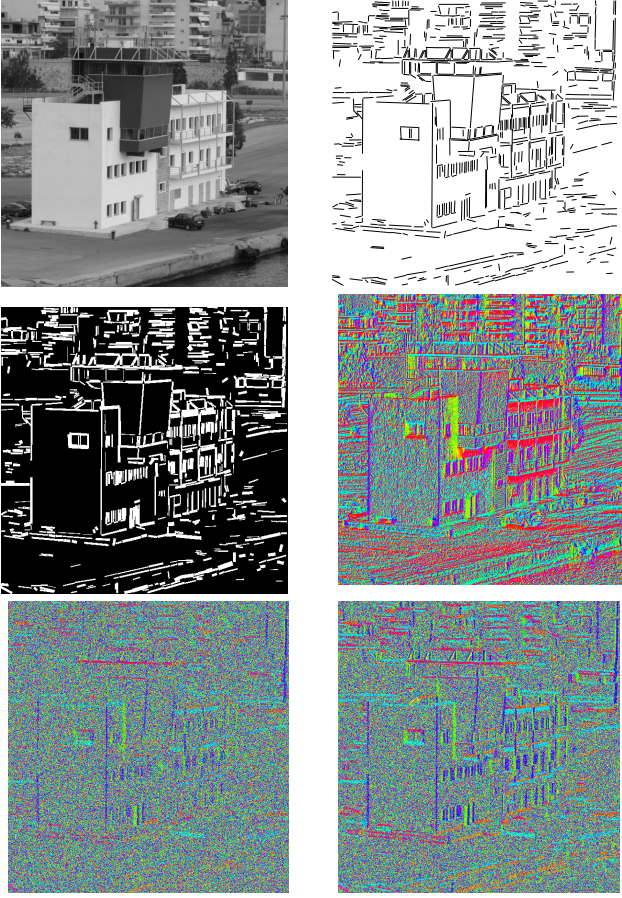
Fig. 6 From left to right, top to bottom: the original Pirée image I^0 of size 600 \times 600 pixels, the output of the LSD, the whole output rectangles of the LSD, the orientation field \theta^0 , a sample from P_0 and a sample from Q_0 .
