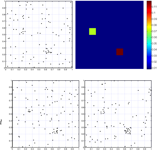
Fig. 4 Top left: the original set of points s^0 with the regions R_i as squares delimited by the dashed lines. Top right: values of p_{Q_0}(R_i) where Q_0 is the maximum entropy distribution in \mathcal{Q} \cap \mathcal{I} given by Equation (9). Bottom : two samples of n = 100 points from the probability distribution Q_0 . These two samples have the same (\varepsilon, U) -meaningful regions as the original set of points s^0 . See the text for more details about the \text{NFA}_U exact values for these regions. One can clearly perceive in the two bottom figures perceptual groups that are similar to the ones of the original set of points.
