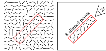
Fig. 5 Example of an orientation field (elementary small segments), a rectangle r (delimited in red), and its aligned points (for a precision p , hence here on the figure \tau = p\pi ). Figure courtesy of R. Grompone von Gioi.
